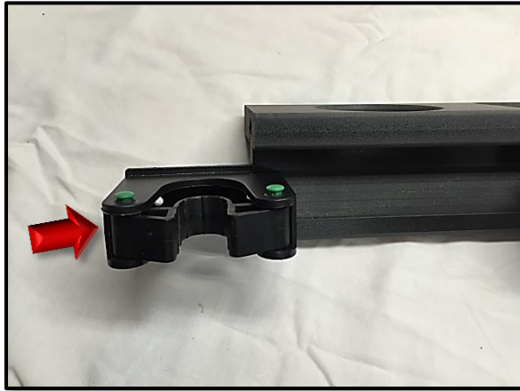
Step 1. Slide the neck grips into the top rail.
